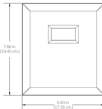
Faceplate - Top View
